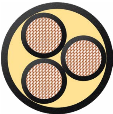
BizLink SeaLine® BWTS cable 3x1x35.0 BK Order no.: L45550-D31-K6
