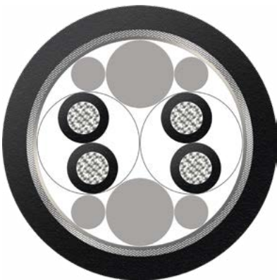
BizLink SeaLine® BWTS cable 2x2x0.75 VZN BK Order no.: L45551-D22-K16
