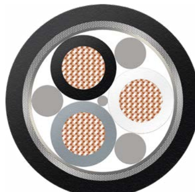
BizLink SeaLine® BWTS cable 3x1x4 BK Order no.: L45551-H31-K6
