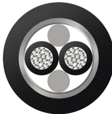
BizLink Sealine® BWTS cable 1x2x0.75 VZN BK 订购号: L45551-D21-K16
