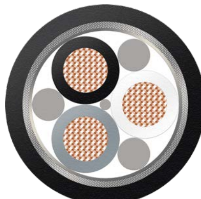
BizLink Sealine® BWTS cable 3x1x4 BK 订购号: L45551-H31-K6
