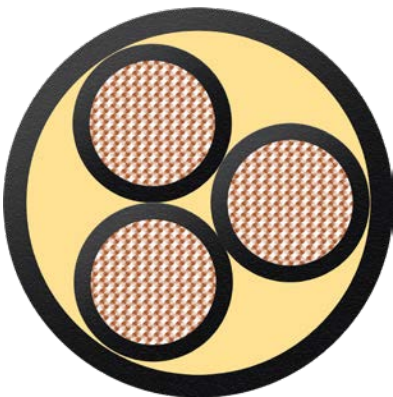
BizLink SeaLine® BWTS Kabel 3x1x35.0 BK Bestell-Nr.: L45550-D31-K6
