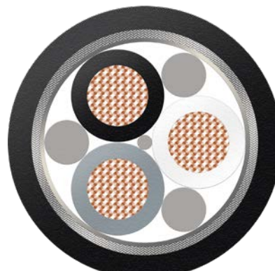
BizLink SeaLine® BWTS Kabel 3x1x4 BK Bestell-Nr.: L45551-H31-K6
