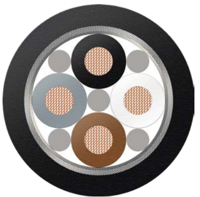
BizLink SeaLine® BWTS cable 4x1x1.5 BK Order no.: L45551-F41-K16
