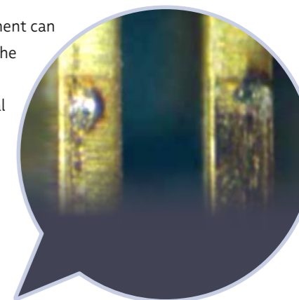
Contact melting in connection technology - here an RJ45 terminal (IEC 62652)
